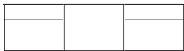
CR9-208-4 Six Drawer Two Center Door Credenza Case: W108 D20.5 H29.25
