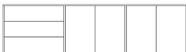
CR9-208-7 Three Drawer Four Door Credenza Case: W108 D20.5 H29.25
