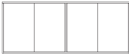
CR9-202 / -203 / -402 / -403 Four Door Credenza Case: W72 D20.5 H29.25 (-403 One Soft Close Drawer behind each set of doors)
