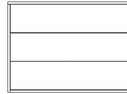
CR9-702 / -412 Three Drawer Chest Case: W40 D20.5 H29.25
